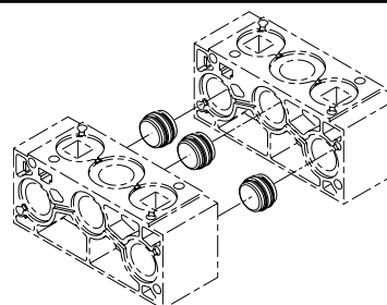
4-Way Isolator Plugs IEM Stackable
