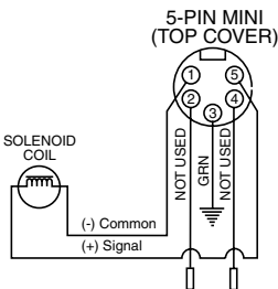
5-Pin Male/Single Solenoid (Encl. Option N, Wiring Option F)
