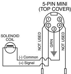
5-Pin Male/Single Solenoid (Encl. Option N, Wiring Option G)
