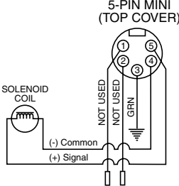
5-Pin Male/Single Solenoid (Encl. Option N, Wiring Option C)
