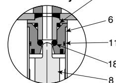
Continuous Duty Pilot Only
