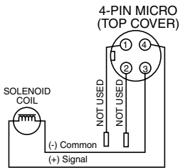
4-Pin Male/Single Solenoid (Encl. Option J, Wiring Option F)
